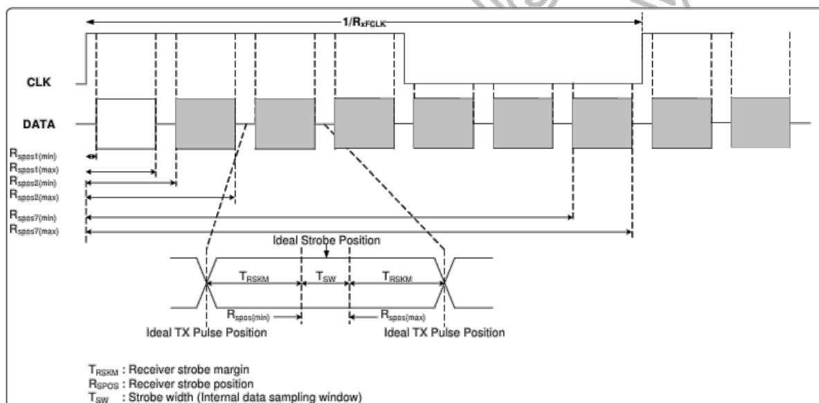
Figure 10.1: LVDS figure
